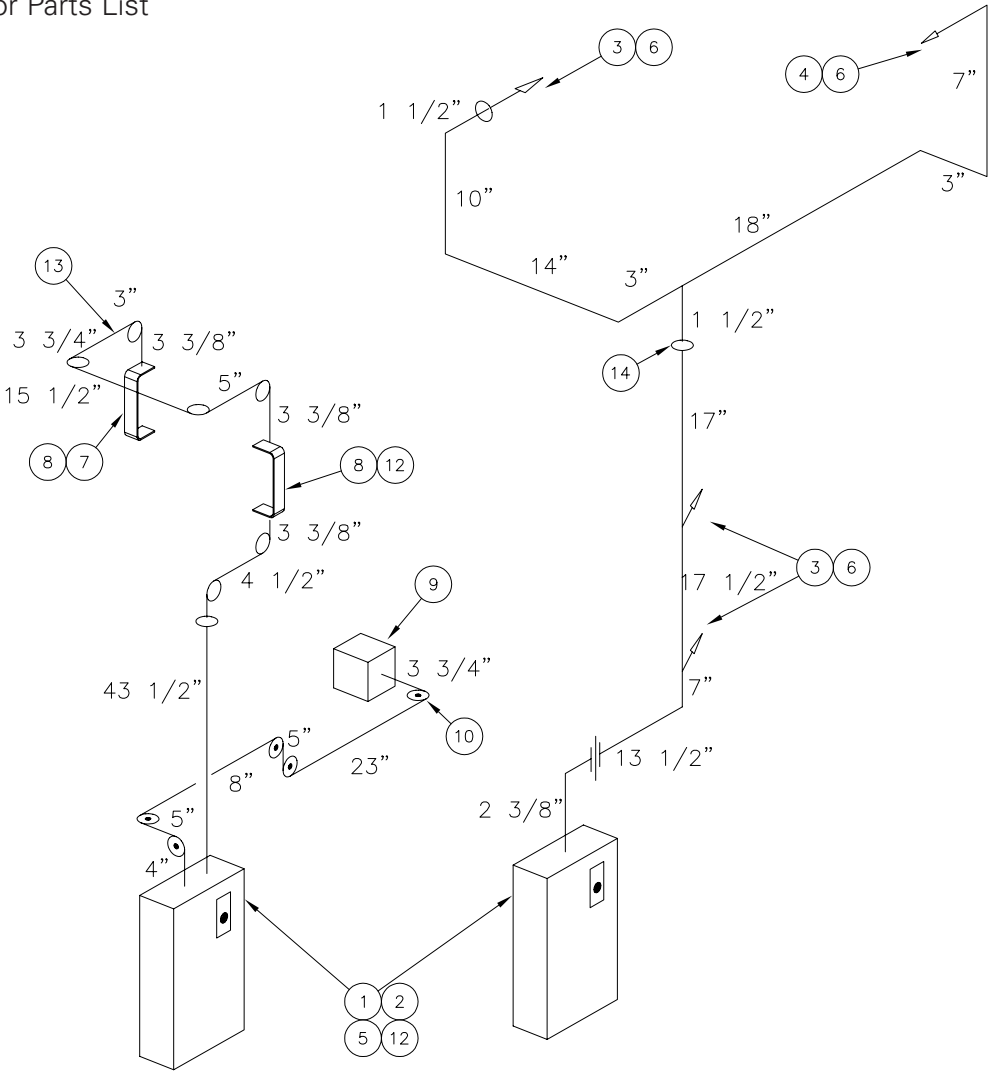
ISOMETRIC VIEW
