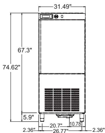
NBCF99/59-8A FRONT VIEW
