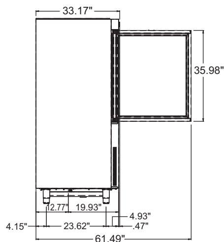
NBCF99/59-8A SIDE VIEW
