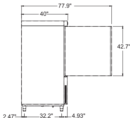
NBCF115/55-16A NBCF220/110-16A SIDE VIEW
