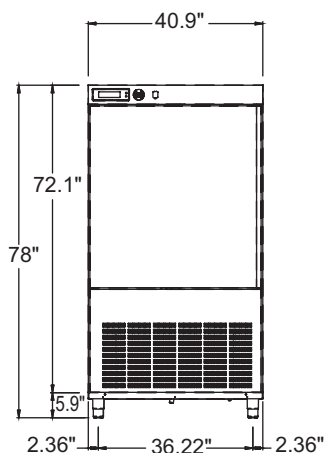
NBCF115/55-16A NBCF220/110-16A FRONT VIEW
